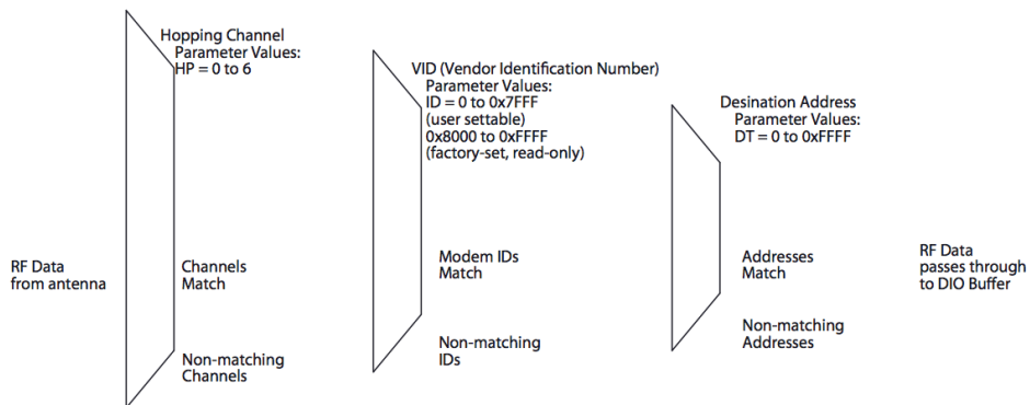
Filtration layers contained in the RF packet header
